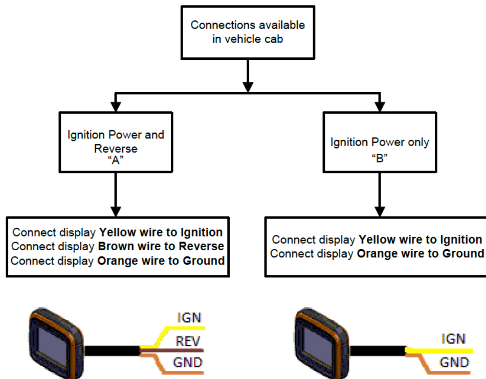
Figure 1. Electrical Connections
