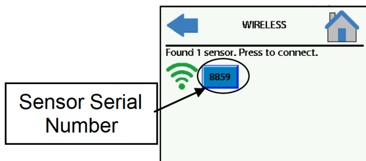
Figure 7. Wireless Connect Screen
