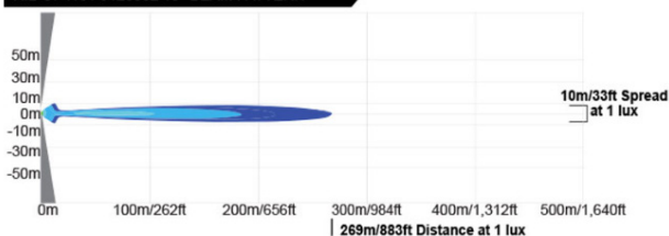
XIL-OP110 / 9123882 10° BEAM PATTERN
