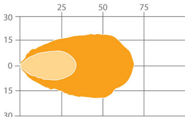
Headlight Beam
