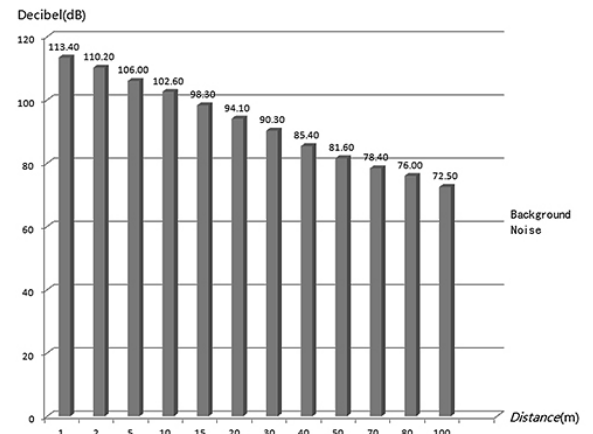
Decibel and Distance Corresponding Curve
