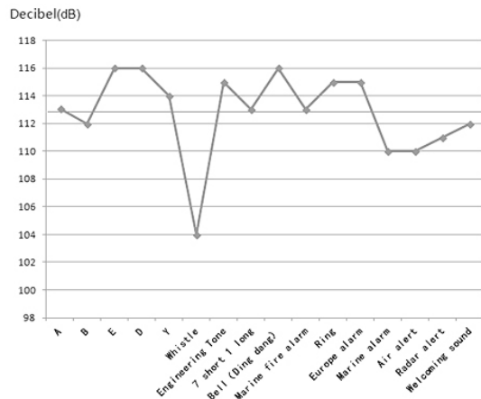
Decibel and Tone Corresponding Curve
