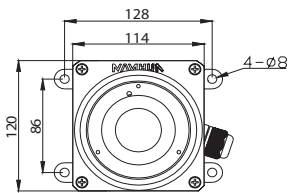
AE310U - Wall-mounted version
