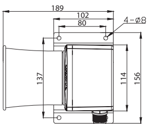
AE310U - Wall-mounted version
