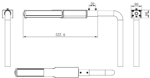
Pole-mount model (LY400-P-22W)
