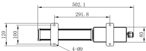
Bulkhead-mount model (LY400-B-22W)
