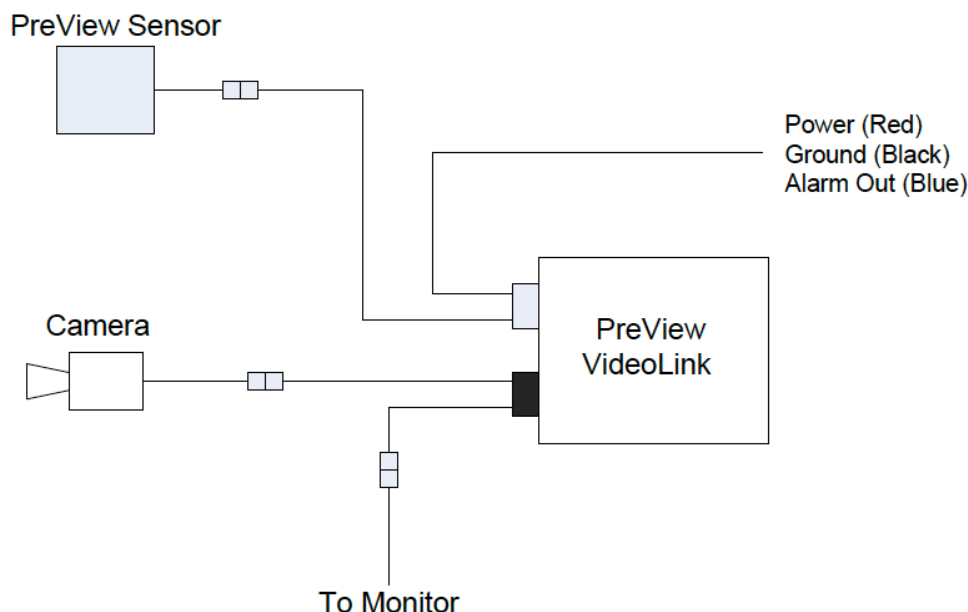
Figure 2. Connections Diagram
