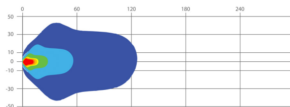
60° Beam Pattern
