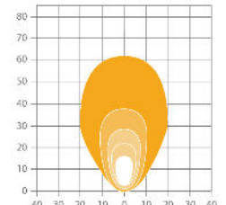
Flood
