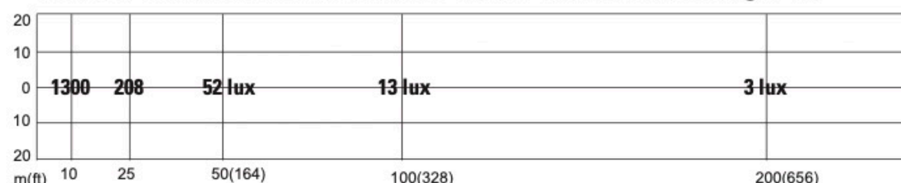
Beam Pattern
