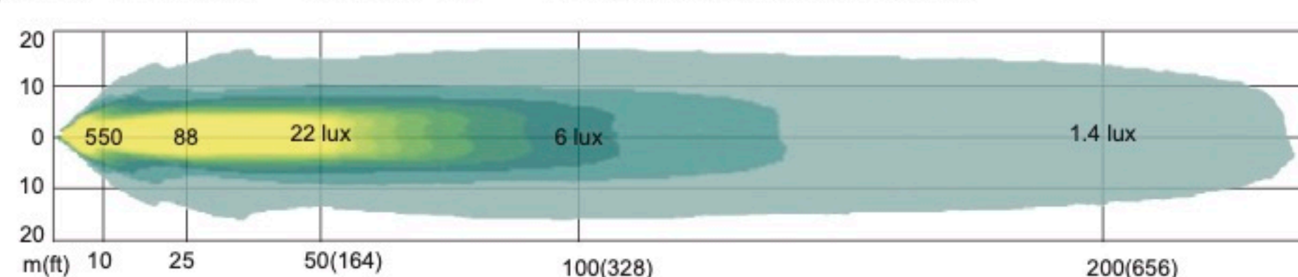
Spot Pattern 55,000 cd 469m/1539ft Max Beam
