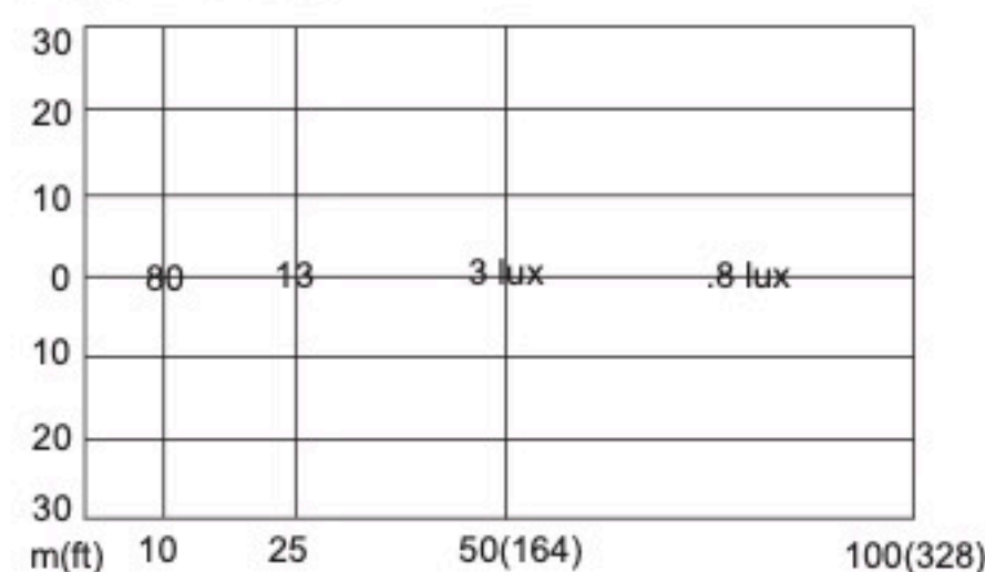
Flood Pattern
