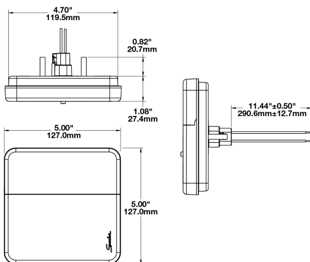
Line Drawings
